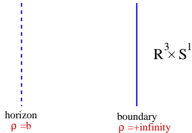
Figure 22: The black brane describing \mathcal{N} = 4 SYM at finite temperature.
